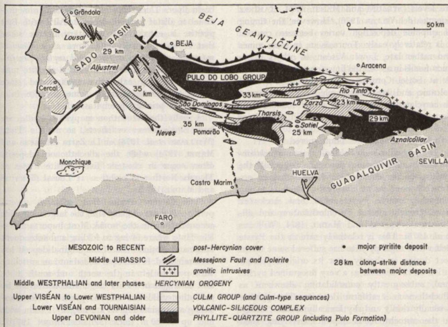
Fig. 5—Geology and major pyrite deposits in the Iberian Pyrite Belt. Note regular spacing of the large deposits. Adapted from CARVALHO et al. (1976)
