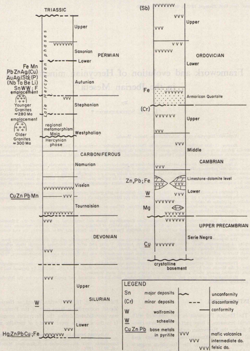
Fig. 1 — Generalized section illustrating timing and evolution of mineralization in the Iberian Meseta
