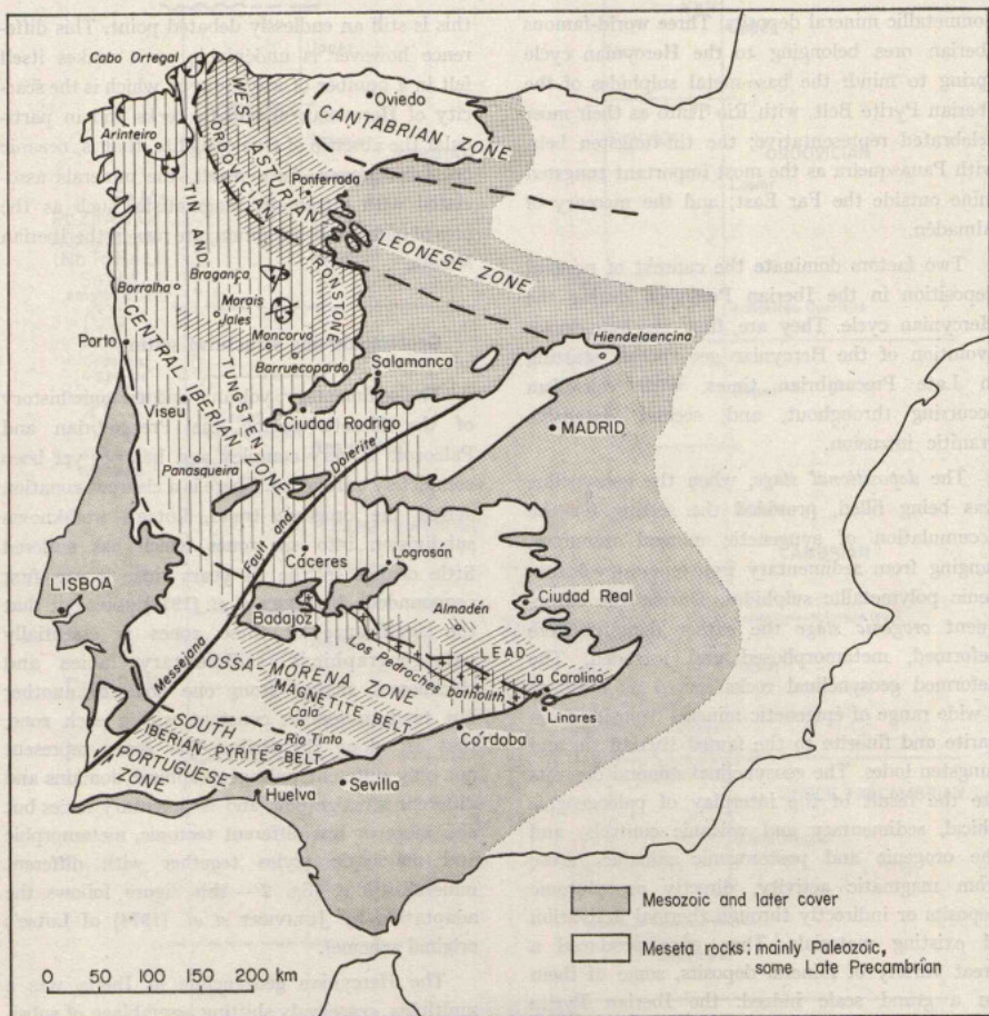
Fig. 2—Principal metallogenetic provinces in the Iberian Meseta
