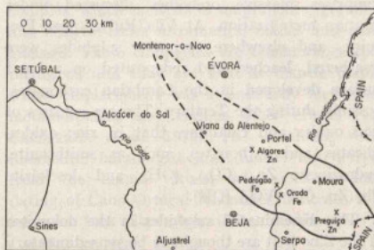
Fig. 3 — The South-Portuguese zinc-magnetite belt, After GOINHAS (1971)
