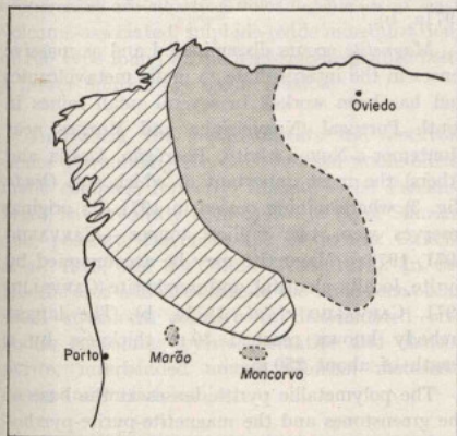
Fig. 4 — Distribution of Lower Ordovician ironstone deposits around an emergent landmass in the northwest Meseta. Stippled: zone in which ironstone occurs; hatched: probable land during Ordovician. After RIBEIRO (1974).
